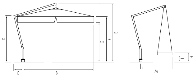
CAPRI ON GROUND ANCHOR WITH EXTENSION PART
